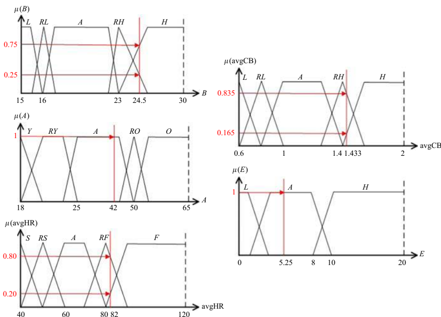
Figure 13. Membership values of input parameters for W0001
